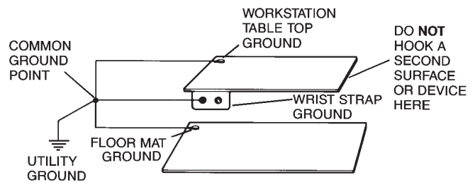
Figure 11. 09740 dual bench mount.
