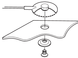
Figure 12. Installing 09814 to mat using supplied hardware.
