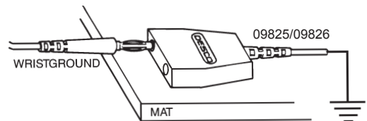
Figure 14. Adding the wriststrap.
