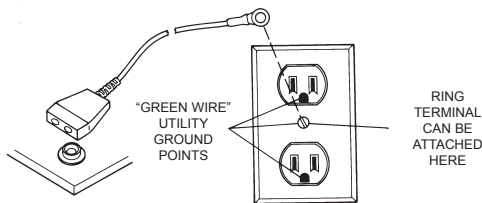
Figure 13. Hooking up ground cords
